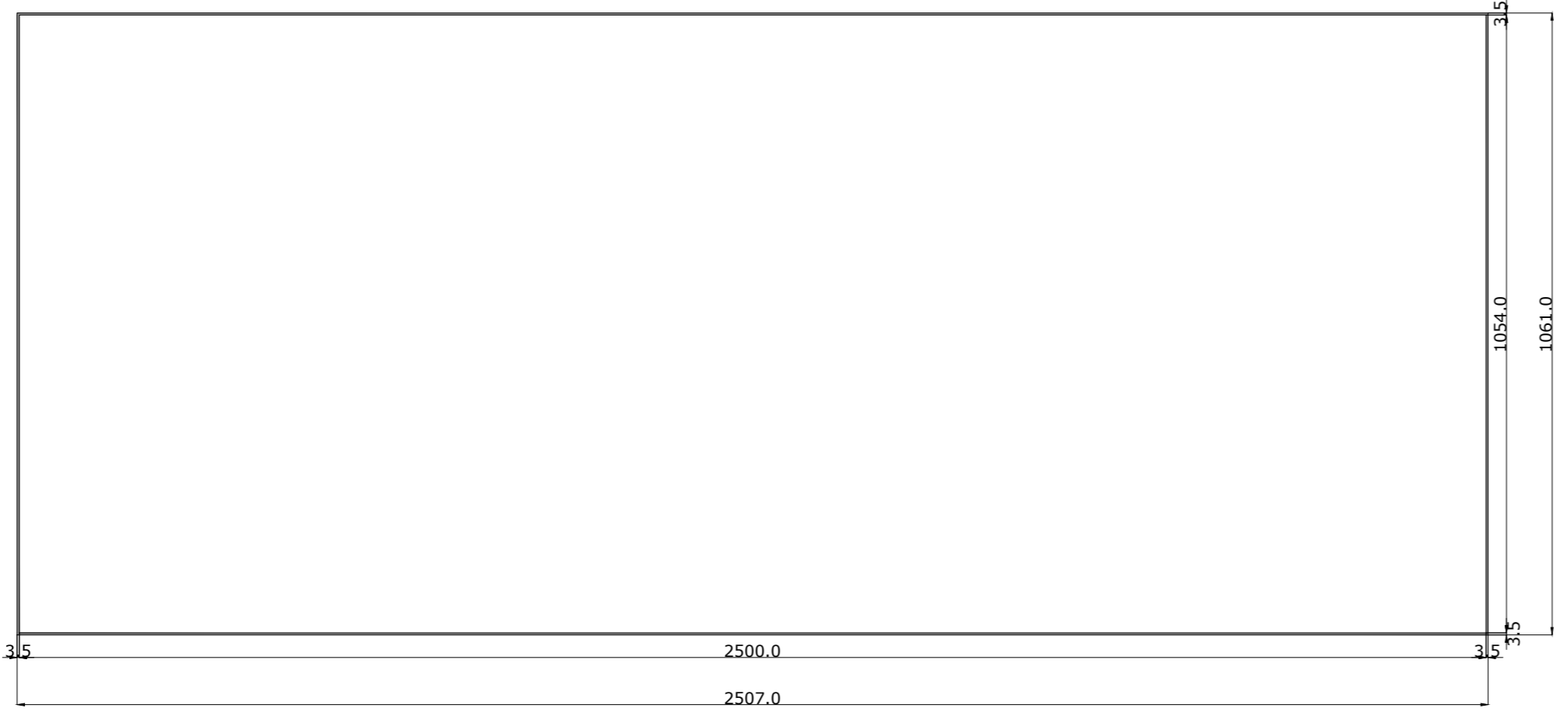
02 ELEVATION A -CBS-HALO-WIDE-2.5 - 2.37
