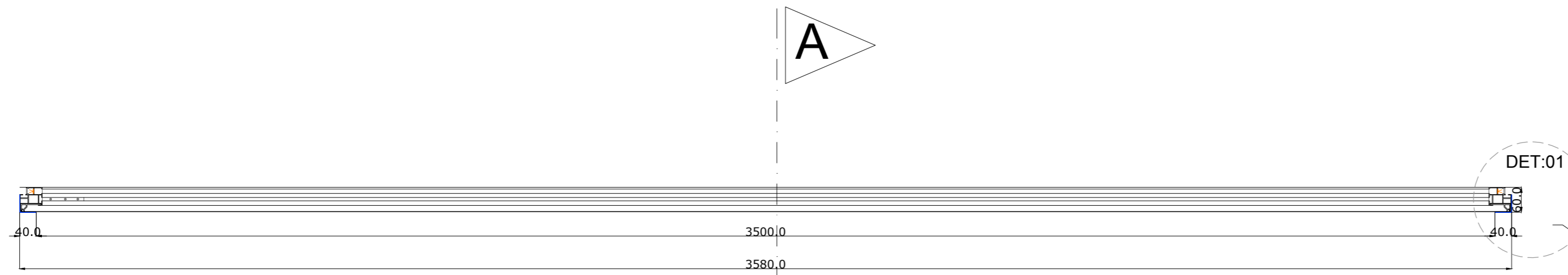
01 BLUEPRINT - CSB-HALO-SLIM-3.5 - 2.37
