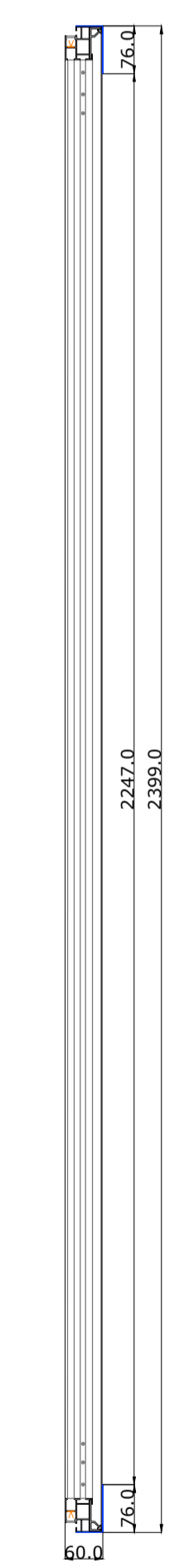
03 SECTION A'A- CSB-HALO-WIDE-1.78
