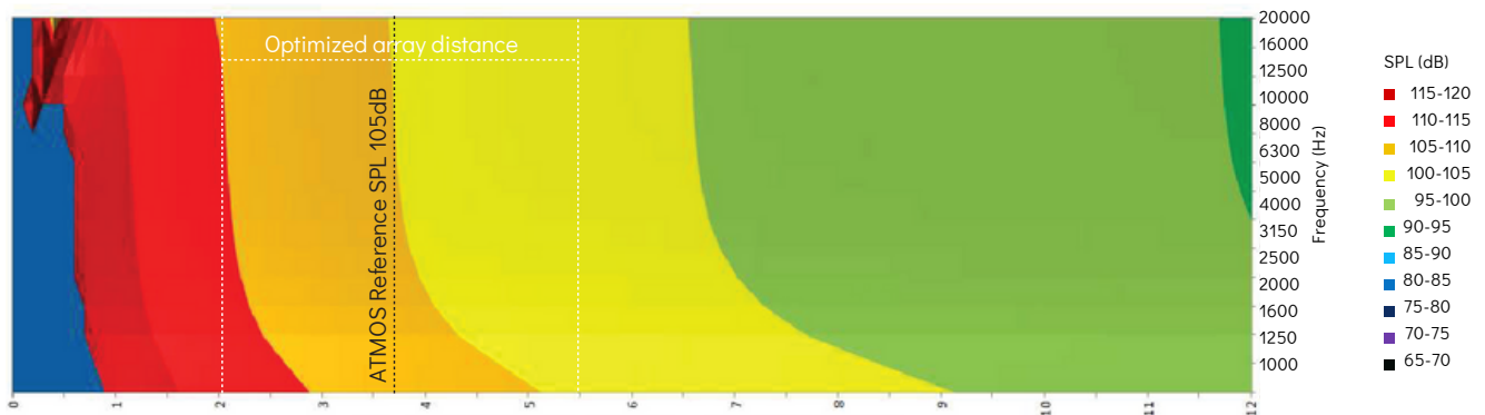
Distance from the array along the central axis (between the two central tweeters) (m). on-axis SPL of the array at distances 0 - 12m
