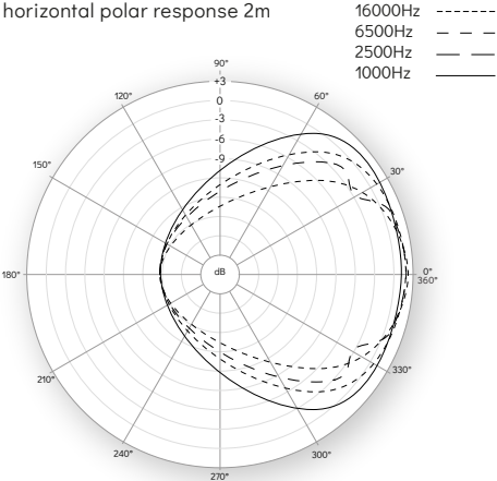
horizontal polar response 2m
