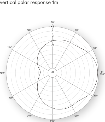
vertical polar response 1m
