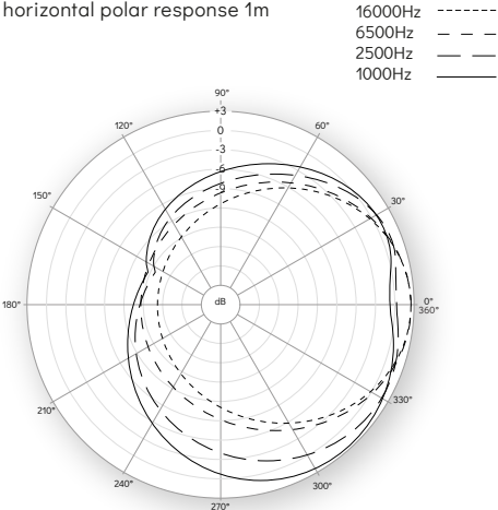
horizontal polar response 1m
