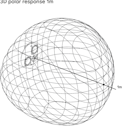
3D polar response 1m
