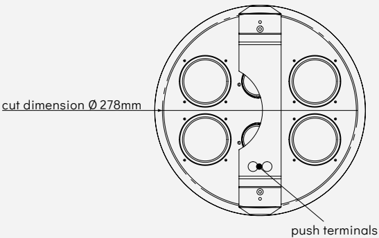
push terminals
